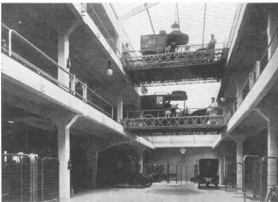
In 1906 the Büro AG Perret, Architects and Engineers, built a parking system that went down in history in the Garage du Rue Ponthieu in Paris. This parking system used a storage and retrieval unit.
